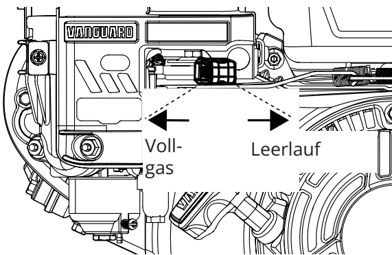
Gashebel
